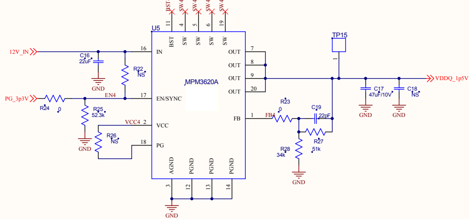
MPM3620A: 1.5V at 2A schematic
