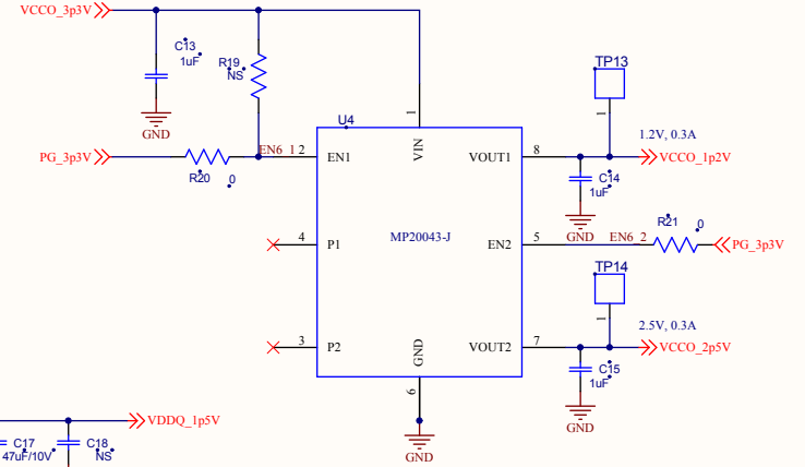
MP20043: 1.2V/2.5V at 300mA each
