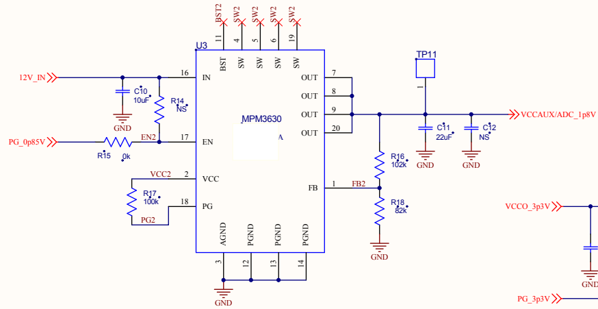
MPM3630: 1.8V at 3A schematic
