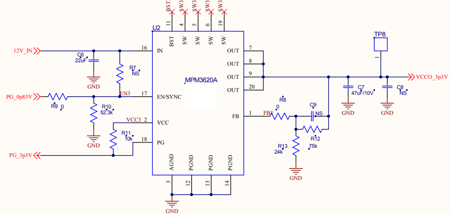
MPM3620A: 3.3V at 2A schematic
