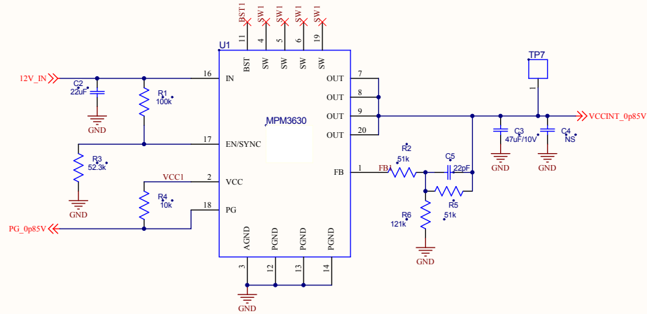
MPM3630: 0.85V at 3A schematic
